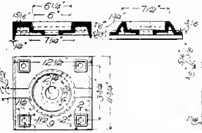
Figs. 4880-82. TRUCK CENTER-PLATE.
